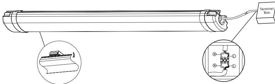
3. Insert the fitting into the hooks.
